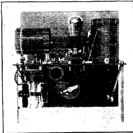
REAR VIEW OF THE SET SHOWING RELATIVE POSITION OF TUNED-CIRCUIT HELICES AND R.F. CHOKES. THE CHOKES CAN BE LOCATED MORE ACCURATELY BY REFERENCE TO THE BOTTOM VIEW
