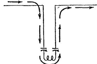
FIG. 3 As folded antenna - 80 meters
