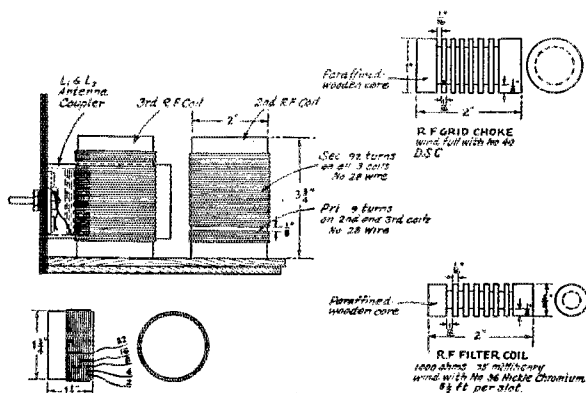
FIG 6 CONSTRUCTION OF THE TUNING COIL AND THE CHOKES
