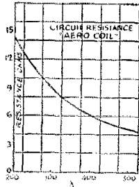
FIG. 4. RESISTANCE-FREQUENCY CURVE OF AN R.F. TRANSFORMER SECONDARY CIRCUIT
