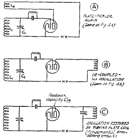
FIG. 7 DEVELOPING THE ARMSTRONG CIRCUIT FROM THE PLATE TICKLER
