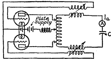
A - BALANCED VALLAURI PLATE DIRECT COUPLED GRIDS INDUCTIVELY COUPLED
