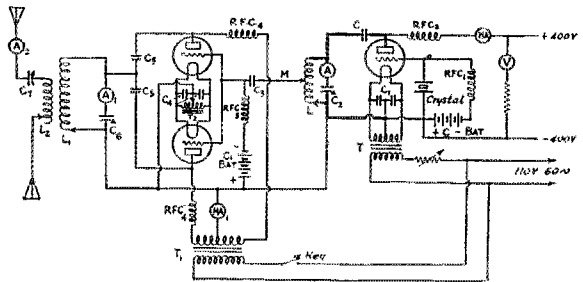
FIG. 1 THE COMPLETE CIRCUIT
