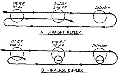
FIG. 5 THE INVERSE DUPLEX ARRANGEMENT SHOWN AGAIN TO EXPLAIN THE NEED FOR THE FILTER SYSTEM
