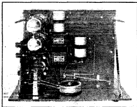
UNDER SIDE OF SHELF, SHOWING R.F. CHOKES, MODULATION CHOKES, MODULATION TRANSFORMER AND INVERTED TUBES
