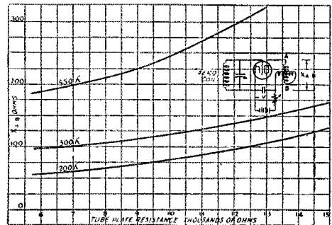
FIG. 6. POSITIVE REACTANCE NECESSARY TO MAKE UX201-A TUBE OSCILLATE Input from coil shown in photograph; plate voltage variable, voltage factor of tube ( \mu ) equal to eight.
