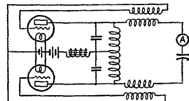
D - BALANCED MODIFIED COLPITTS PLATE CAPACITY COUPLED GRID INDUCTIVELY COUPLED
