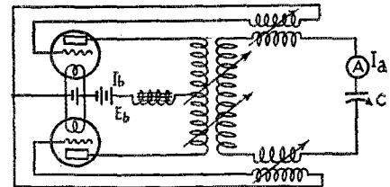
C - BALANCED MEISSNER PLATES & GRIDS INDUCTIVELY COUPLED
