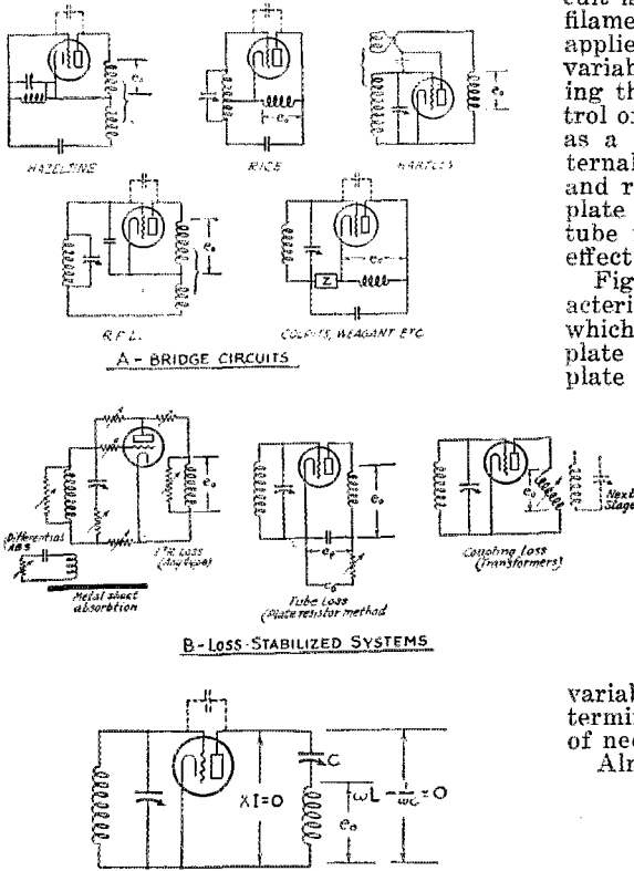
FIG. 2. REPRESENTATIVE EXAMPLES OF STABILIZING METHODS
