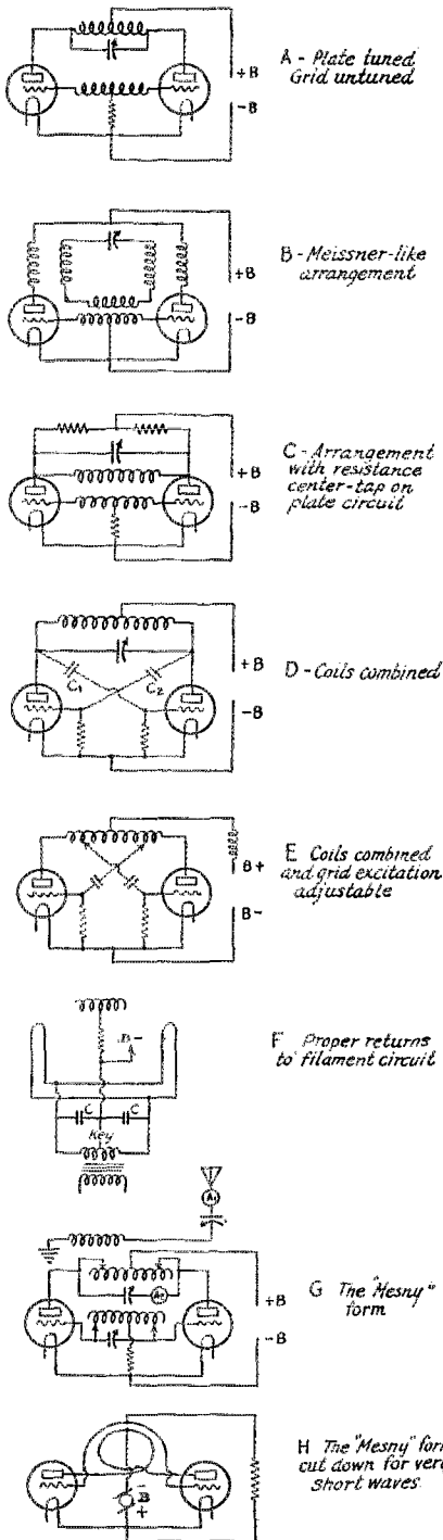
FIG. 13 BALANCED CIRCUITS NOT USING PLATE CHOKER
