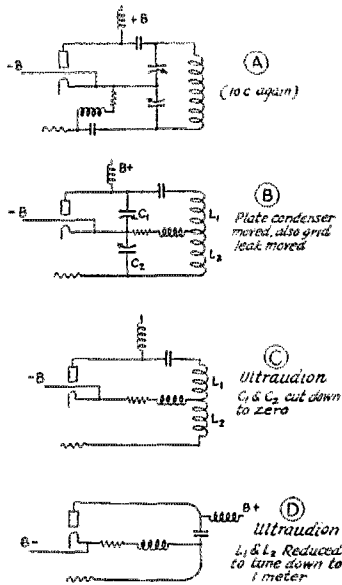
FIG 11 COLPITTS & ULTRAUDION
