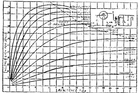
FIG. 5. VARIATION OF GAIN AT DIFFERENT PLATE VOLTAGES AGAINST CHANGES IN THE PRIMARY-SECONDARY RELATION The curves are made for a wavelength of 300 meters but the same principle may be applied at other wavelengths.
