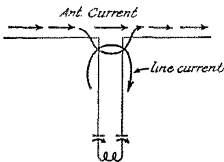
FIG. 2 As top and 2-wire feeder - 40 meters
