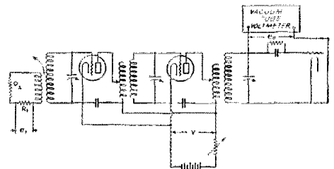
FIG. 8. A MEASUREMENT SET-UP USEFUL IN THE DESIGN OF MULTI-STAGE VOLTAGE-STABILIZED R. F. SYSTEMS
