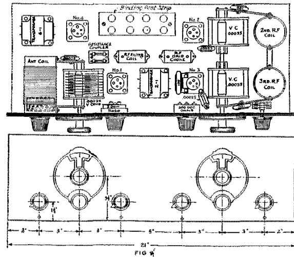
ARRANGEMENT OF PARTS IN THE R. G. S. RECEIVER
